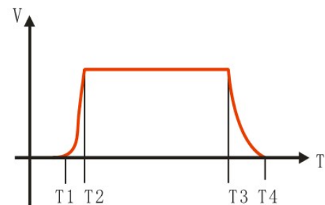
Fig.6b: Analysis chart of working speed and actuator output process of BLDCM
