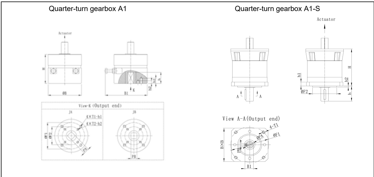
Main dimension
